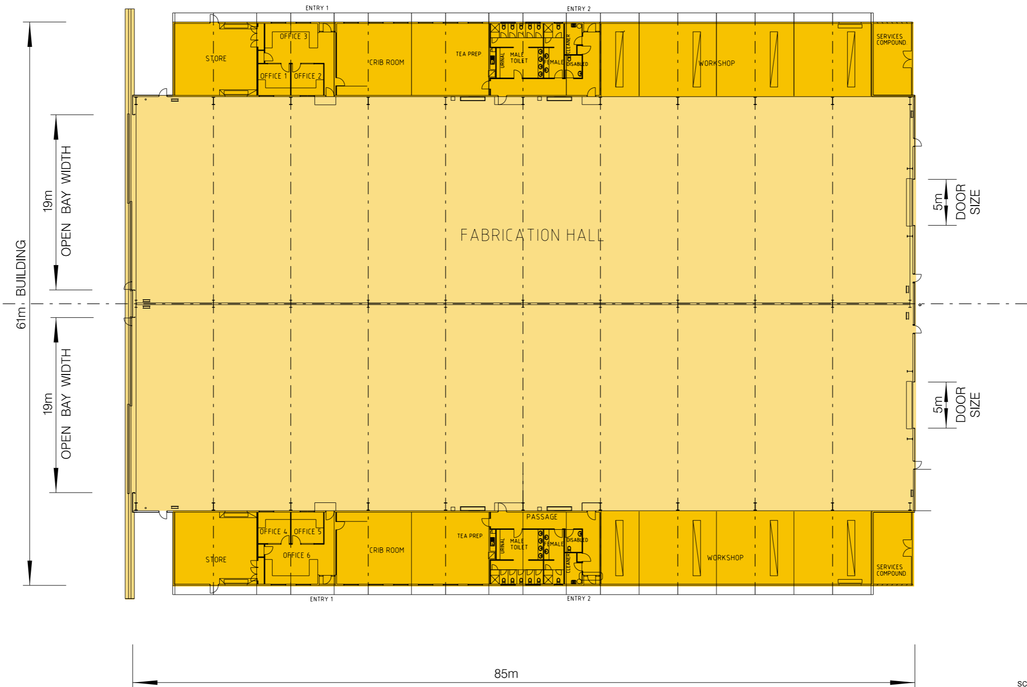
BUILDING 9 FABRICATION HALL No2 - PLAN
