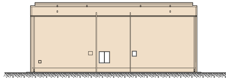
EAST ELEVATION
