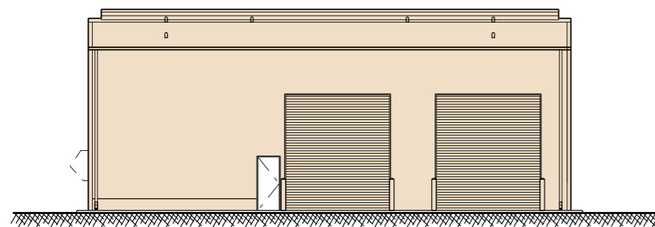
WEST ELEVATION
