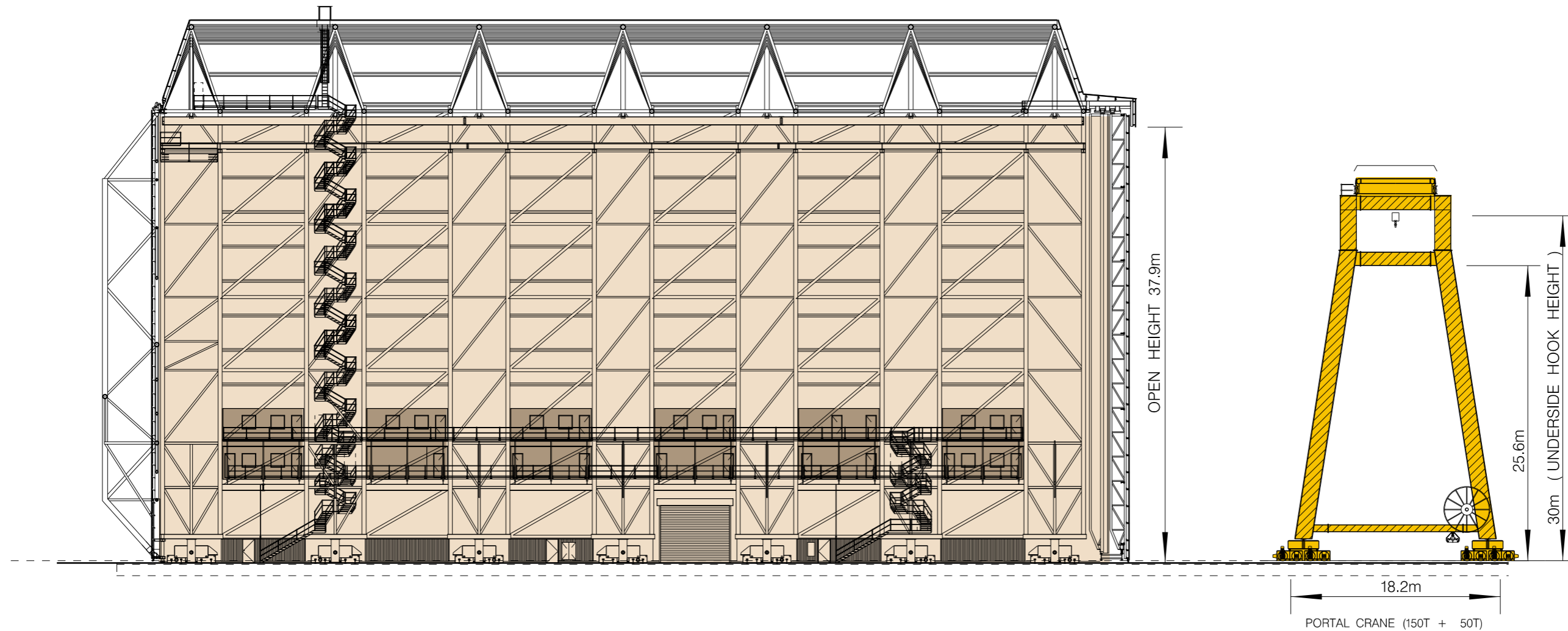
LONGITUDINAL SECTION (SIDE VIEW INSIDE NORTH)
