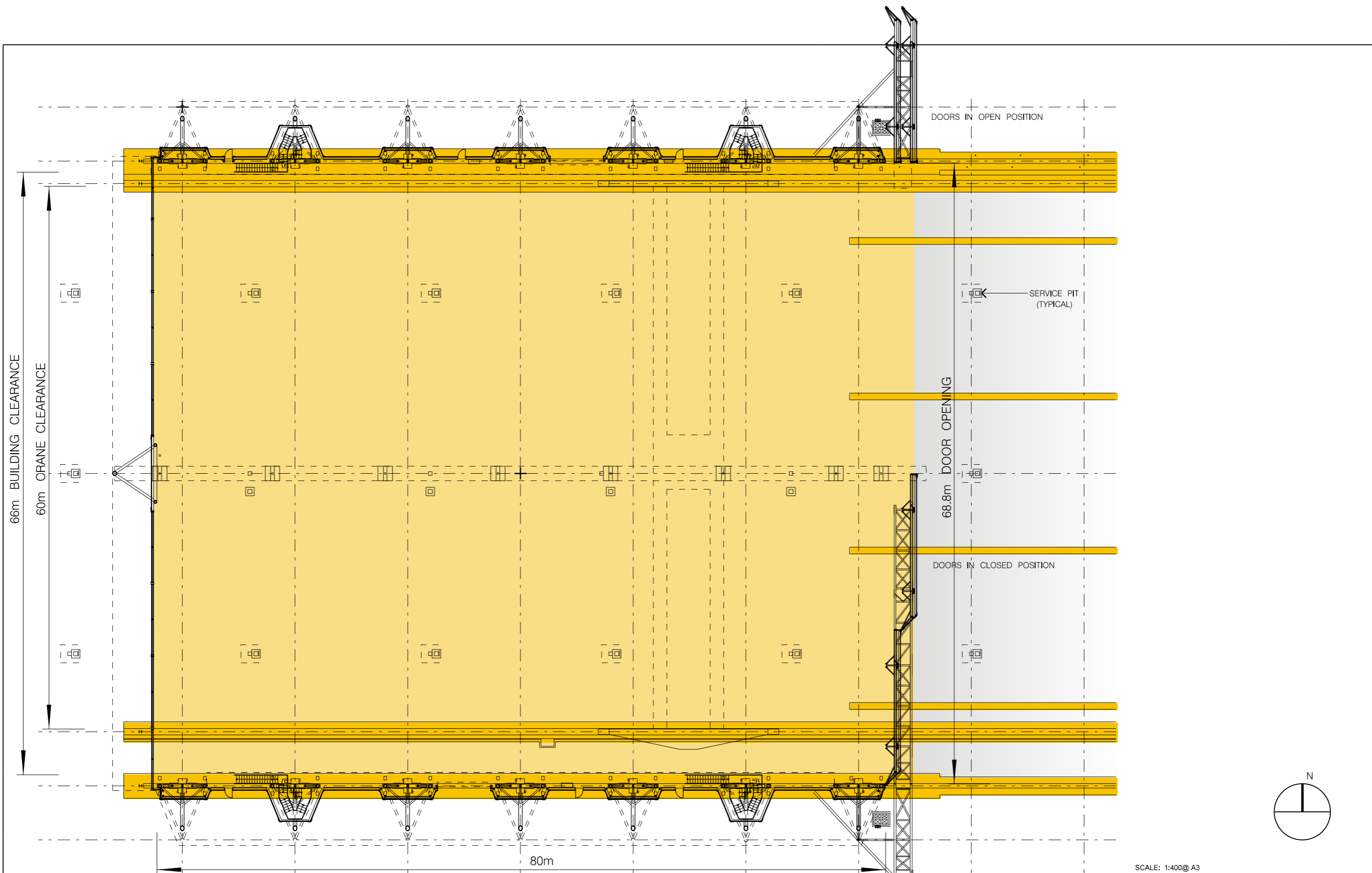
BUILDING 1 MAIN FABRICATION HALL No1 - PLAN
